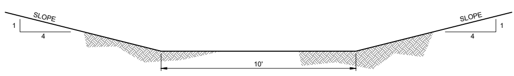
5 DRAINAGE DITCH TYPICAL SECTION 4.1 NOT TO SCALE
