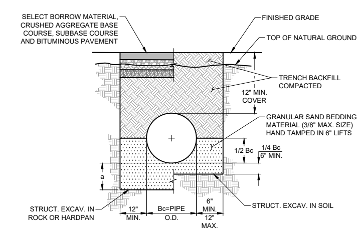
3 PIPE CULVERT BEDDING & BACKFILL DETAIL 4.1 NOT TO SCALE
