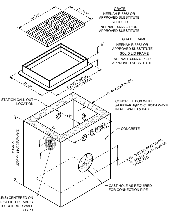
1 STORM DRAIN INLET 4.1 NOT TO SCALE
