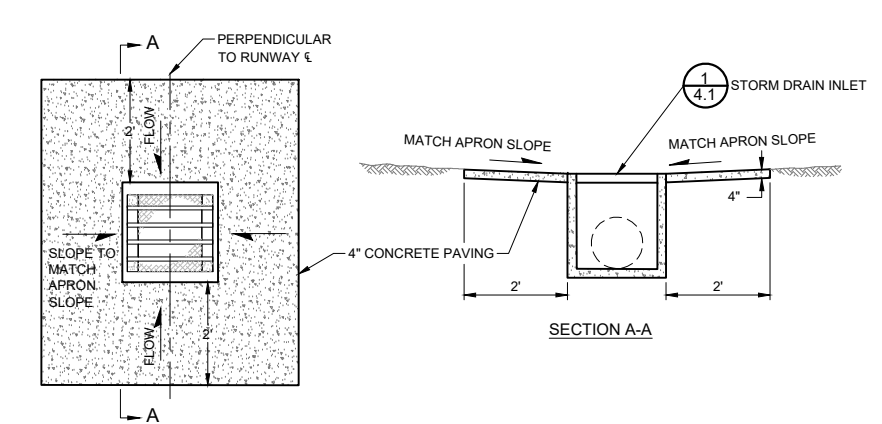
4 INLET APRON PAVING 4.1 NOT TO SCALE
